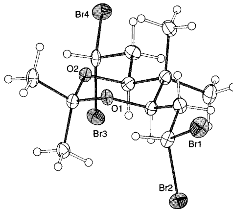
Figure 1. X-ray crystal structure of compound 7
