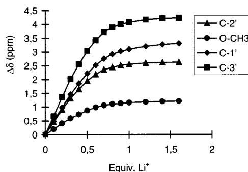
Figure 2. NMR titration of compound 8 with LiBPh 4 ; changes in the 13 C NMR chemical shifts
